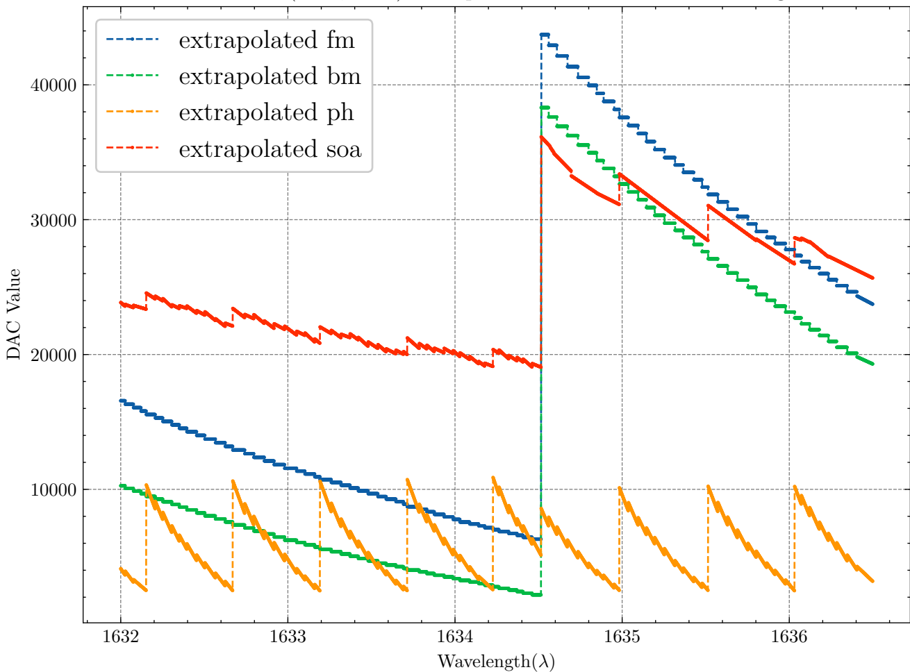
DAC Parameters (1000, 2000) Extrapolated with 3 Intermediate Integer Values
